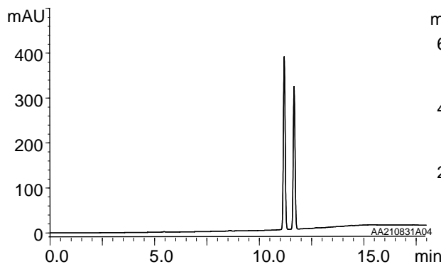
DMT-dA(Bz)-CE phosphoramidite (dA)
