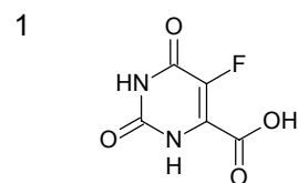
5-Fluoroorotic acid
