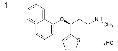
Duloxetine hydrochloride ( S )-Duloxetine hydrochloride
