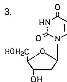
Deoxyuridine
