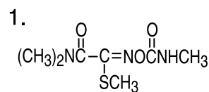
Oxamyl
