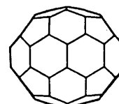
(5,6)-Fullerene(C70)
