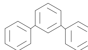
m -Terphenyl
