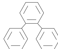
o -Terphenyl
