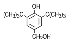
4-Hydroxymethyl-2,6-di-tert-butylphenol (HMBP)
